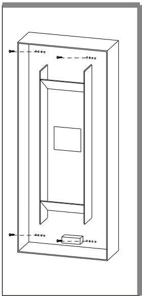
Cleat Mounting
